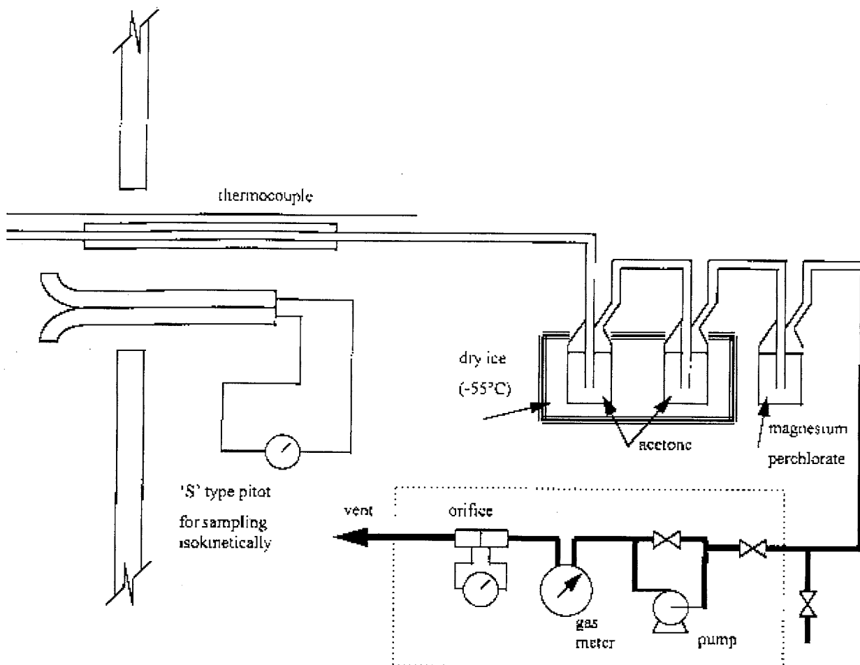
Figure 4.3. Sampling train used by CRE Group, Ltd. (1997)
