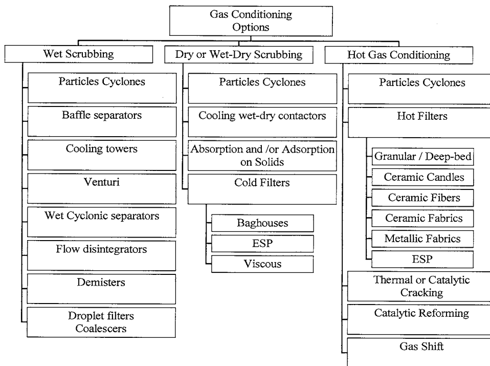
Figure 6.1. Gas cleaning technologies.
