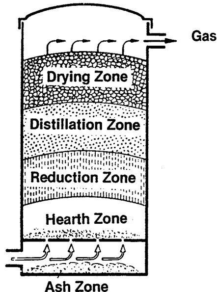
FIG. 9: DIAGRAM OF UPDRAFT GASIFICATION
