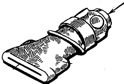
Fig. 41 WATERCOOLED RECTANGULAR NOZZLE FOR CROSSDRAFT GASIFICATION
