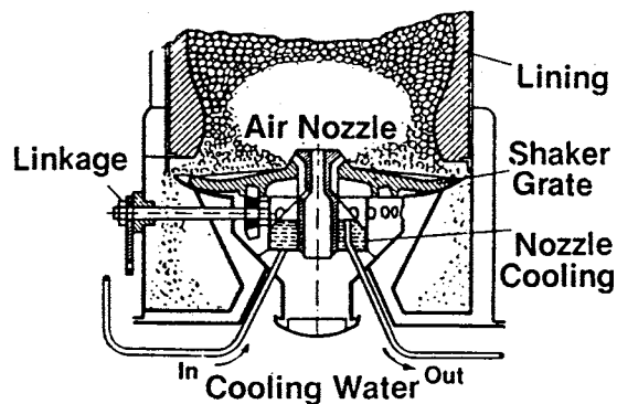
FIG. 34 SHAKER GRATE
